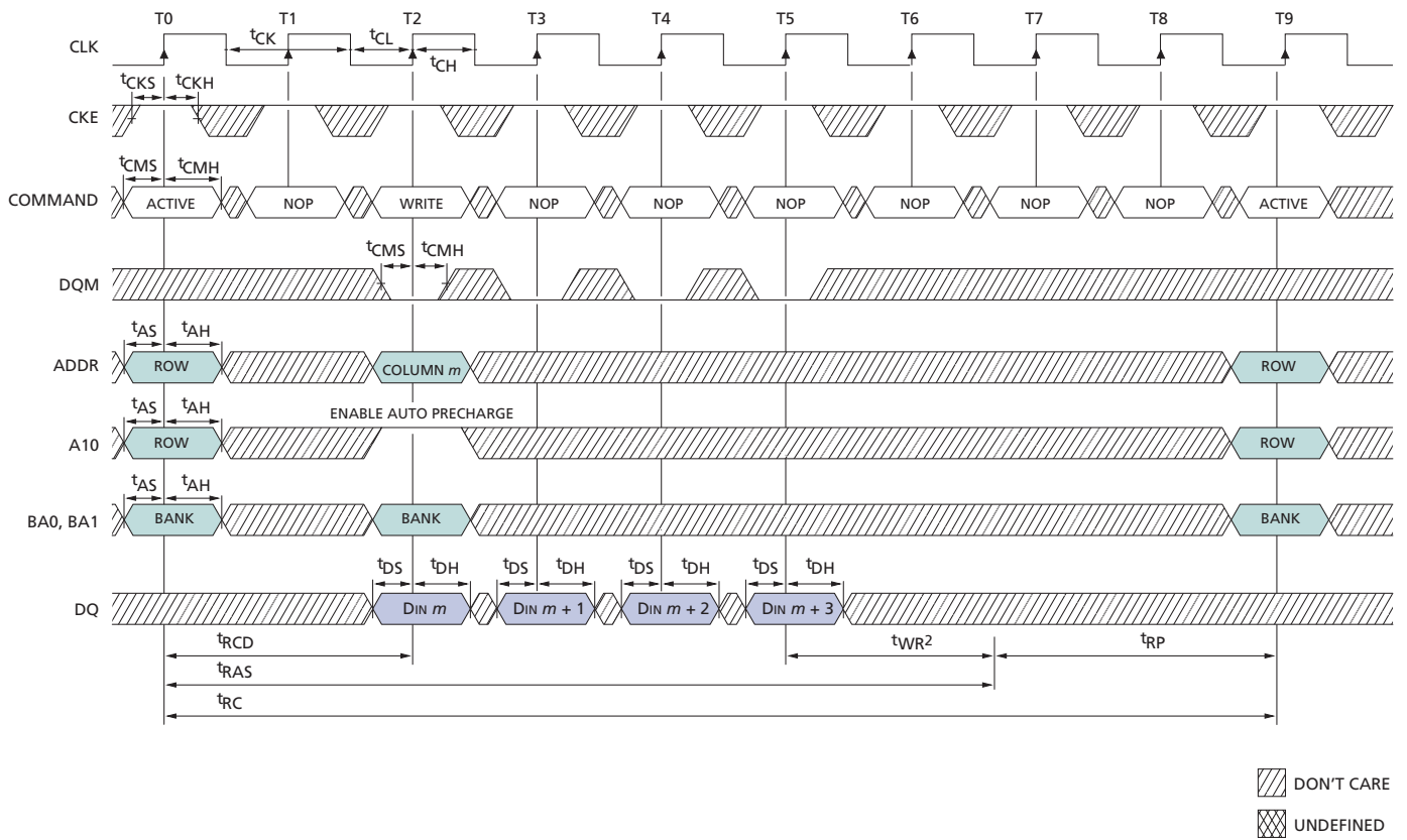
Figure 47: WRITE – with Auto Precharge
